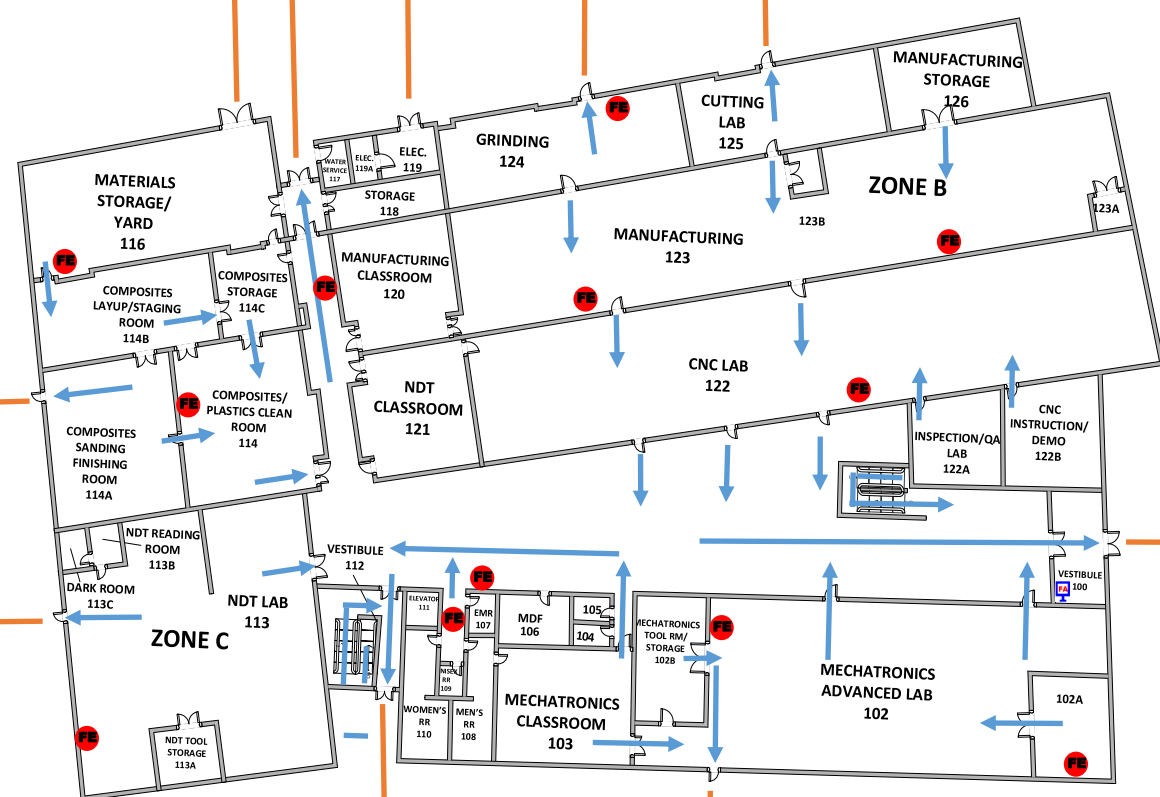
FIRE EXITS 1ST FLOOR
