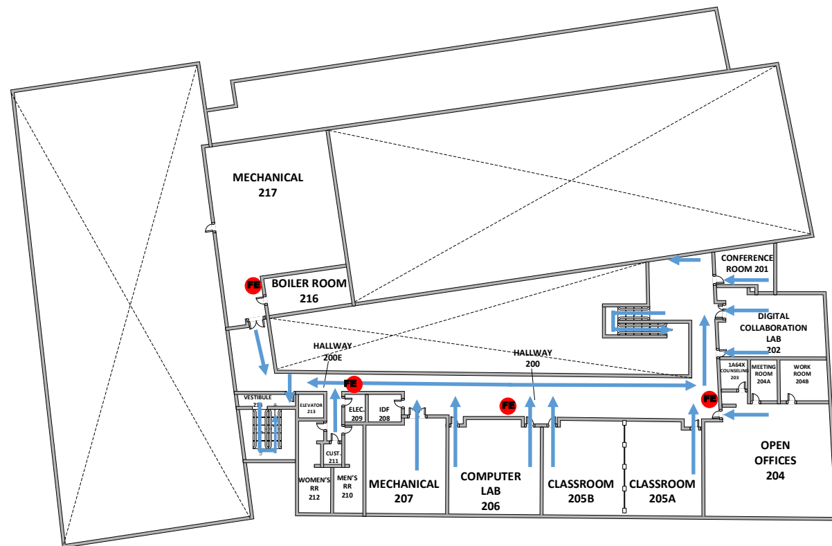
FIRE EXITS 2ND FLOOR
