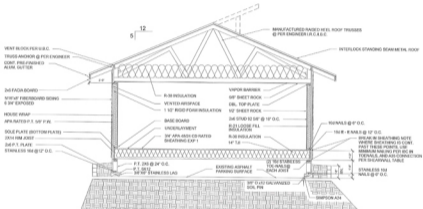
WALL SECTION
